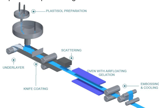
Figure 3: Process flow diagram (coating)
